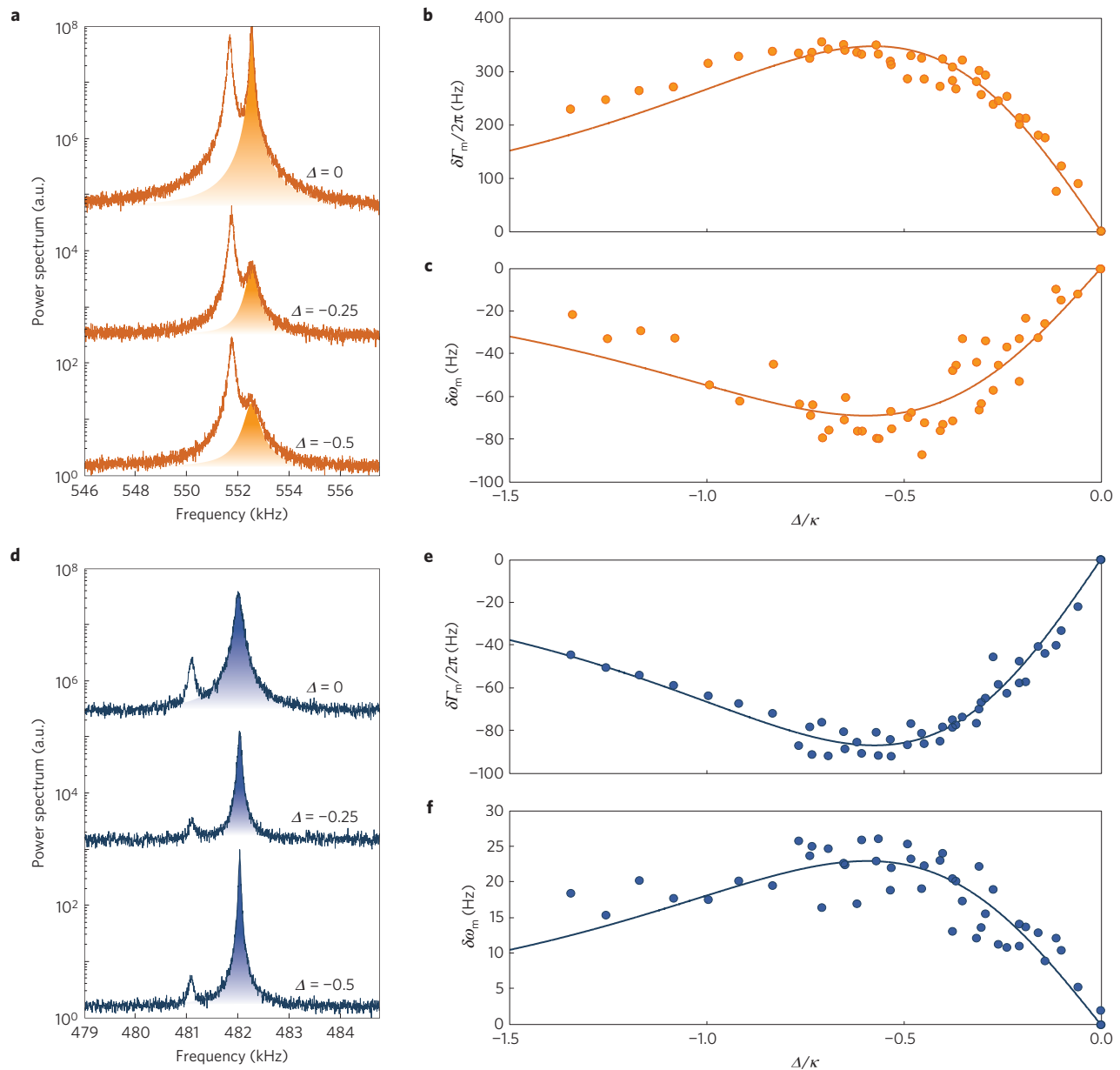
Figure 4 | Optomechanical heating and cooling of two third sound modes. Detuning the optical field results in cooling ( a ) or heating ( d ) of the superfluid excitations. The laser is red-detuned with respect to the cavity for both the 552.5 kHz mode and the 482 kHz mode. Whether the mode experiences heating or cooling depends on the relative magnitude of the radiation pressure force and the sign of the photothermal constant ( \beta ), which itself depends on the optical and mechanical mode. a , Spectra of two closely spaced mechanical modes around 552.5 kHz with varying optical detuning. The shaded mode experiences photothermally induced broadening ( \beta > 0 ), with the mechanical linewidth increasing with increasing red detuning. b,c , Change in mechanical damping rate and mechanical resonance frequency as a function of detuning for the 552 kHz mode. A maximum relative frequency shift of \delta\omega_m/2\pi = -60 Hz is measured at \Delta = -0.60\kappa . Solid line: theoretical fit to photothermal broadening. d , Spectra of two closely spaced mechanical modes around 482 kHz with varying optical detuning. The shaded mode experiences photothermally induced narrowing ( \beta < 0 ), with the mechanical linewidth decreasing with increasing red detuning. e,f , Change in mechanical damping rate and mechanical resonance frequency as a function of detuning for the 482 kHz mode. A maximum relative frequency shift of \delta\omega_m/2\pi = 23 Hz is measured at \Delta = -0.60\kappa . Solid line: theoretical fit to photothermal narrowing. Traces in a and d are offset for clarity. All detuning measurements were taken with 200 nW of launched optical power.
